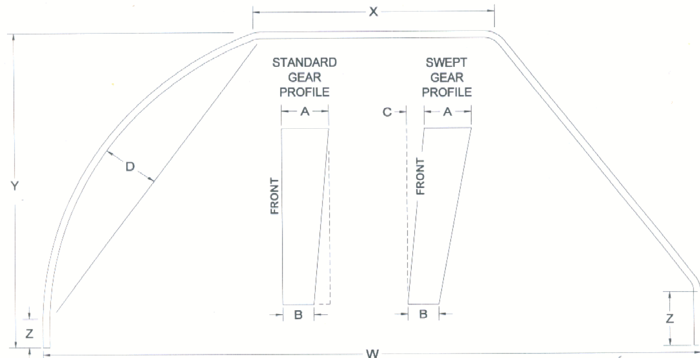
Gear Dimensional Data
